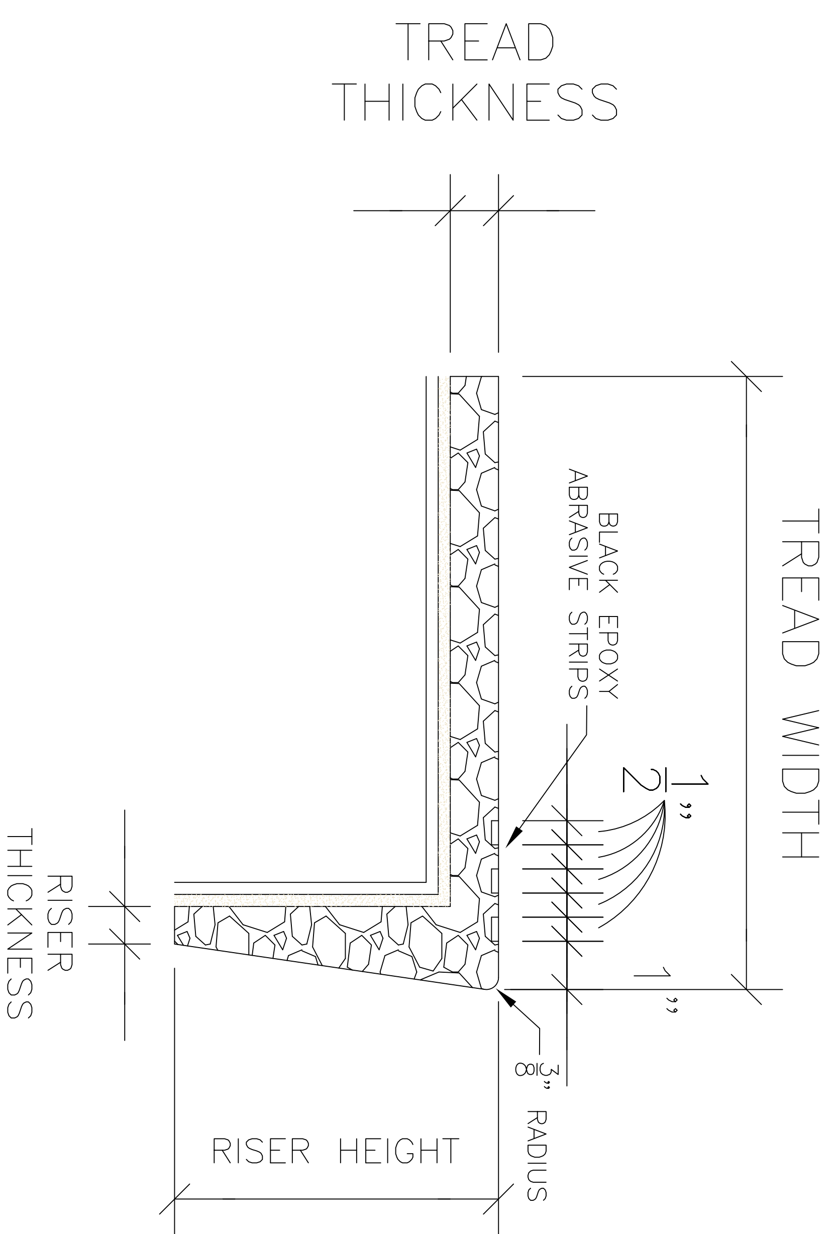
TREAD AND RISER COMBO SECTION SCALE: 6" = 1'-0"
