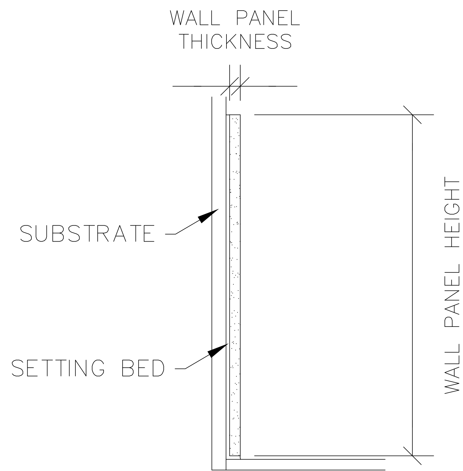
WALL PANEL SECTION Scale: 6" = 1'-0"
