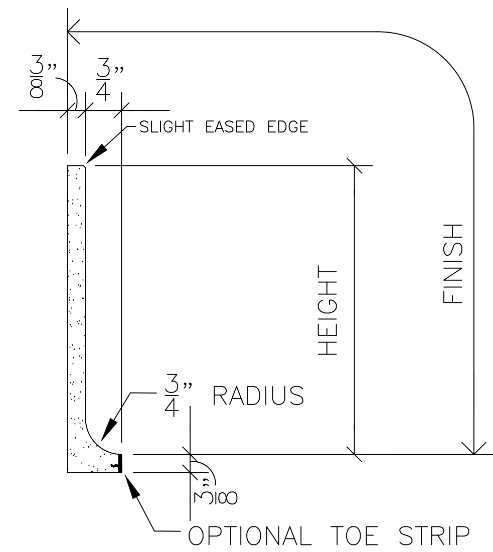
COVE BASE SECTION
